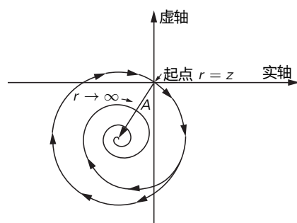
图 30.12: \int_z^\infty \eta e^{-i\omega r/c} dr
